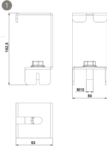
Cable Tray and Wall Hanger Set
