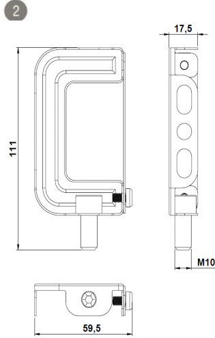
Busbar Hanger Set
